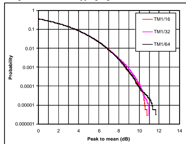
Figure 1: Test Model 1/64 CCDF curve
