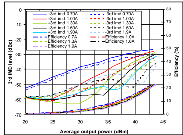
Figure 10: IMD with 2 x W-CDMA source
