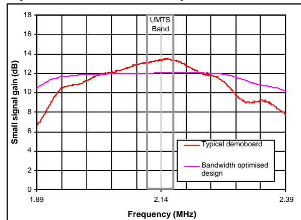
Figure 6: Small Signal Gain
