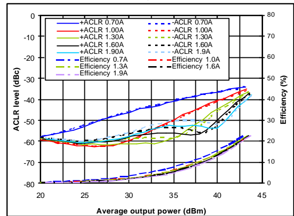
Figure 11: ACLR (lower carrier) with 2 x W-CDMA source
