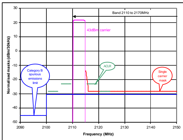
Figure 3: Single Carrier UMTS spectrum requirements
