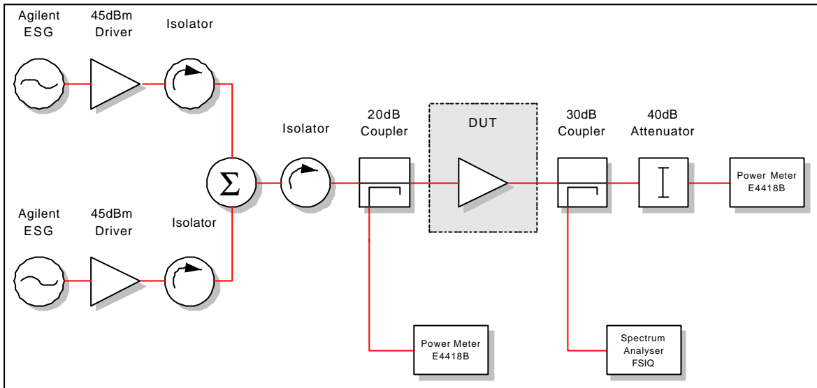
Figure 2: Typical IMD/ACLR test setup
