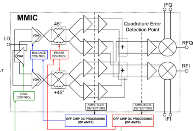
Fig. 3: MMIC Architecture
